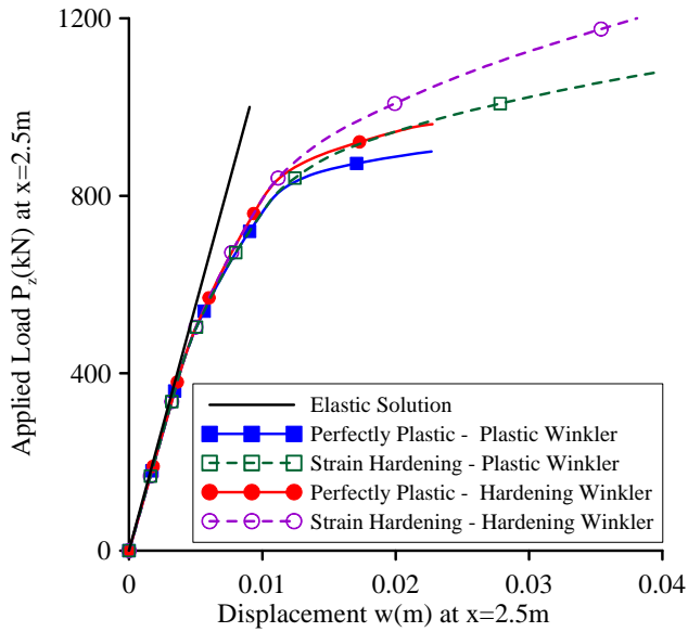
Figure 13: Load – displacement curve at the loading point of the beam of example 3 resting on nonlinear foundation.
