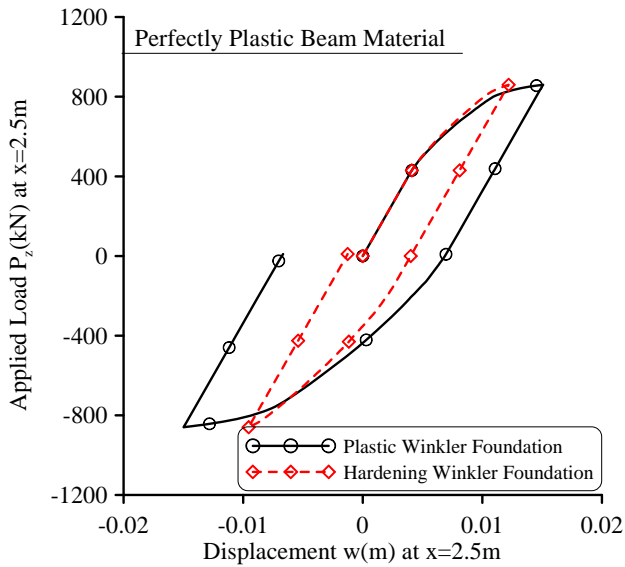
Figure 14: Load – displacement curve at the loading point of the beam of example 3, in case of elastic-perfectly plastic beam material.
