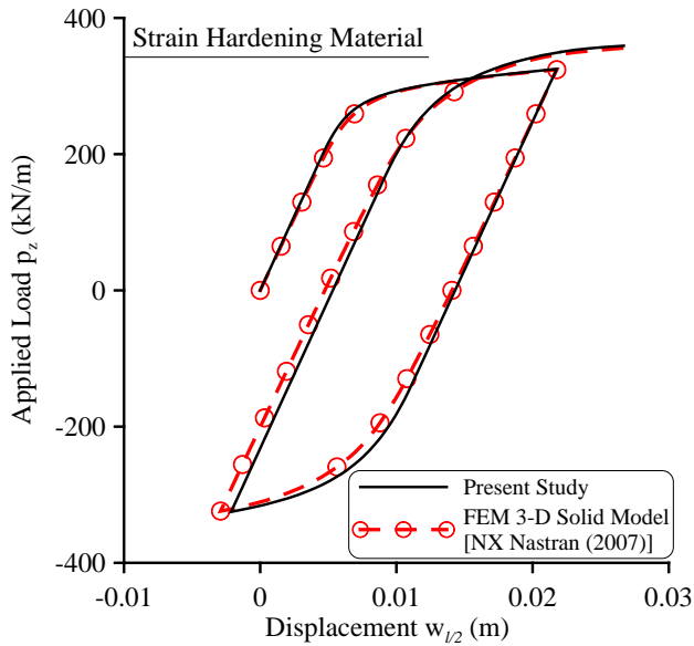
Figure 6: Load – displacement curve at the midpoint of the beam of example 1, in case of elastoplastic-strain hardening material.
