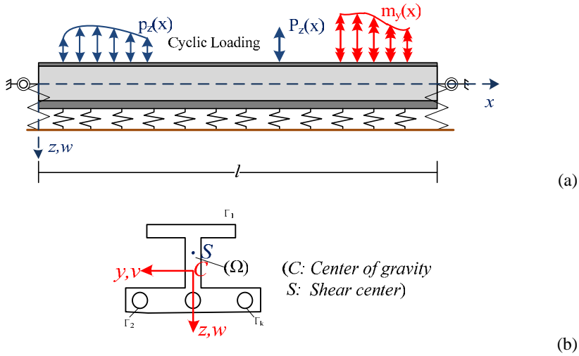
Figure 1: Prismatic beam resting on an inelastic foundation subjected to cyclic bending loading (a) with an arbitrary cross-section having at least one axis of symmetry, occupying the two dimensional region \Omega (b).
