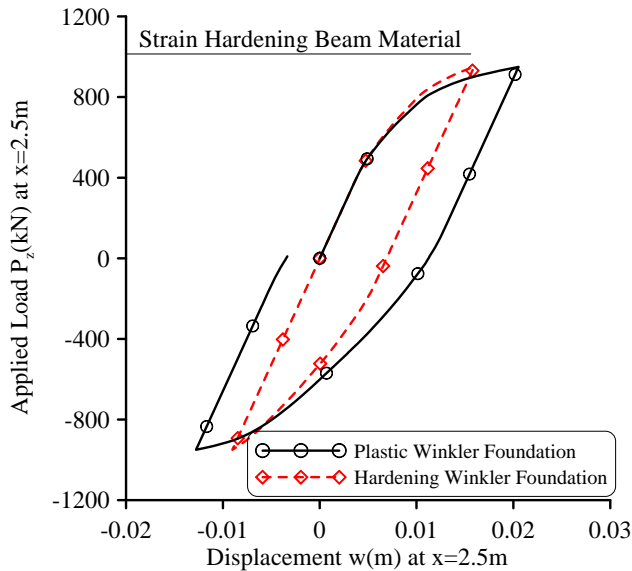
Figure 15: Load – displacement curve at the loading point of the beam of example 3, in case of elastoplastic-strain hardening beam material.
