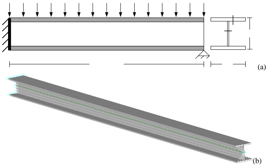
Figure 9: Fixed pinned beam subjected to a uniformly distributed cyclic loading (a) and shell model FEM mesh [NX Nastran (2007)] (b).
