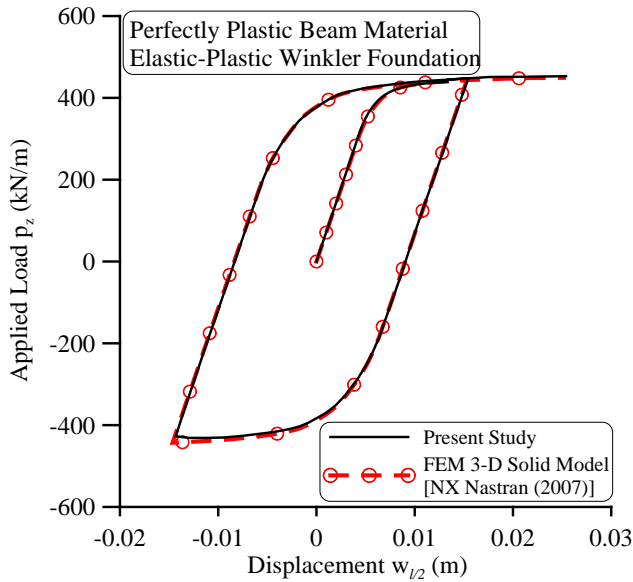
Figure 7: Load – displacement curve at the midpoint of the beam on elastic-plastic Winkler foundation of example 1, in case of elastic-perfectly plastic beam material.
