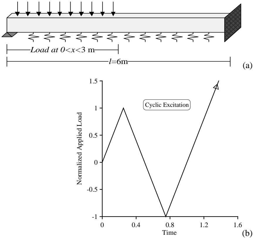
Figure 4: Pinned-fixed beam resting on an elastic-plastic Winkler foundation (a) subjected to a uniformly distributed cyclic loading (b).
