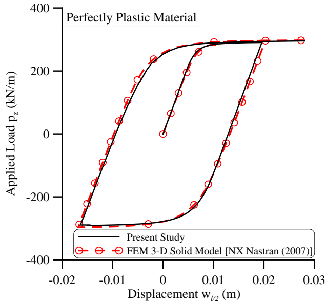
Figure 5: Load – displacement curve at the midpoint of the beam of example 1, in case of elastic-perfectly plastic material.
