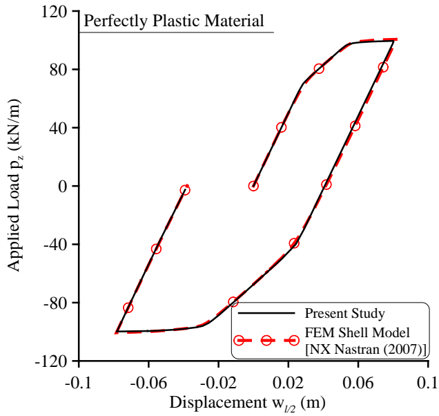
Figure 11: Load – displacement curve at the midpoint of the beam of example 2, in case of elastic-perfectly plastic material.
