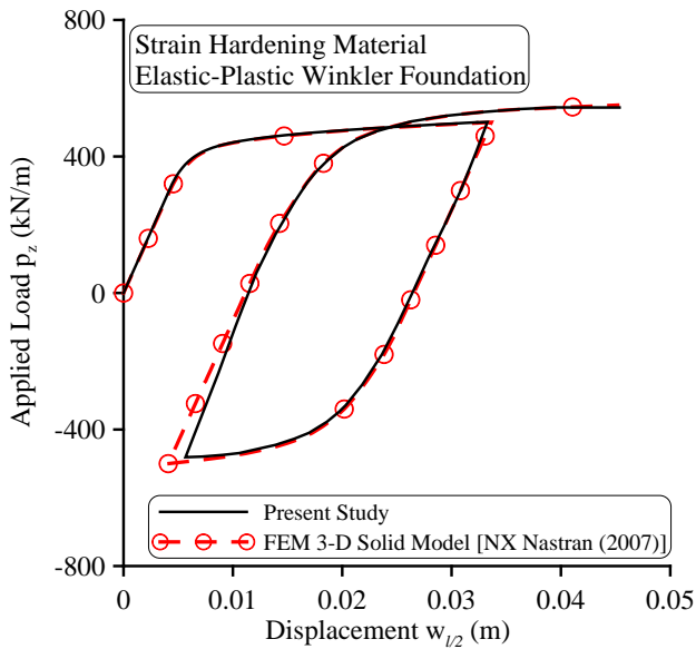
Figure 8: Load – displacement curve at the midpoint of the beam on elastic-plastic Winkler foundation of example 1, in case of elastoplastic-strain hardening beam material.
