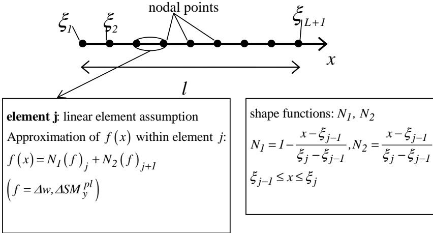
Figure 3: Discretization of the beam interval into linear elements, distribution of the nodal points and approximation of several quantities.
