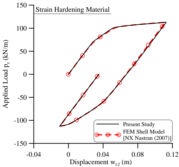
Figure 12: Load – displacement curve at the midpoint of the beam of example 2, in case of elastoplastic-strain hardening material.
