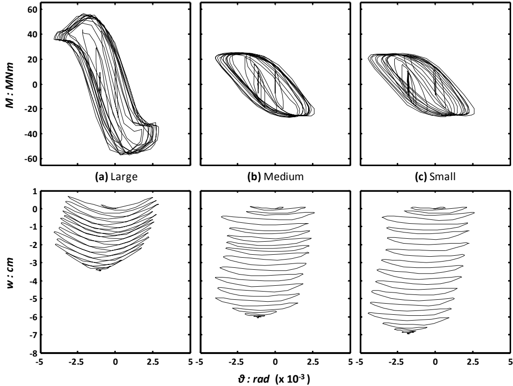
Figure 7. Foundation response to base excitation of a 12-cycle 2 Hz sine pulse with 0.50 g acceleration amplitude (Sin2-0.50 g). Moment–rotation and settlement–rotation response for : (a) the large foundation (FSv = 7.3) ; (b) the medium foundation (FSv = 3.5) ; and (c) the small foundation (FSv = 2.3).
