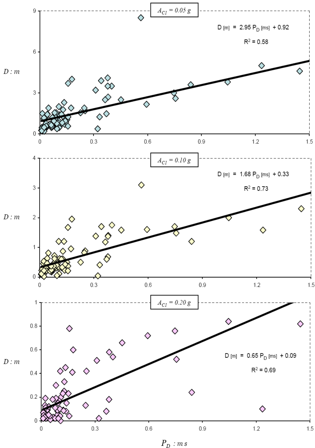
Figure 4. The influence of potential destructiveness factor P_D (as defined by Araya and Saragoni, 1984) on sliding displacement D , for three levels of critical yielding acceleration A_C : 0.05 g, 0.1 g, and 0.2 g
