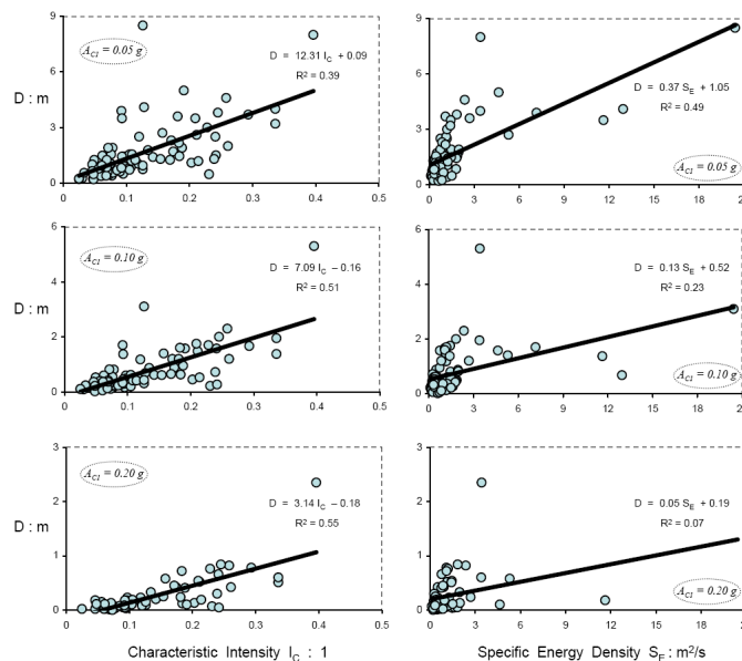
Figure 7. Influence of the dimensionless parameter of characteristic intensity, I_C , on slippage, D , at the left hand-side and effect of specific energy density, S_E , at the right. Observe the poor correlation of the induced slippage with the energy density value of each earthquake event
