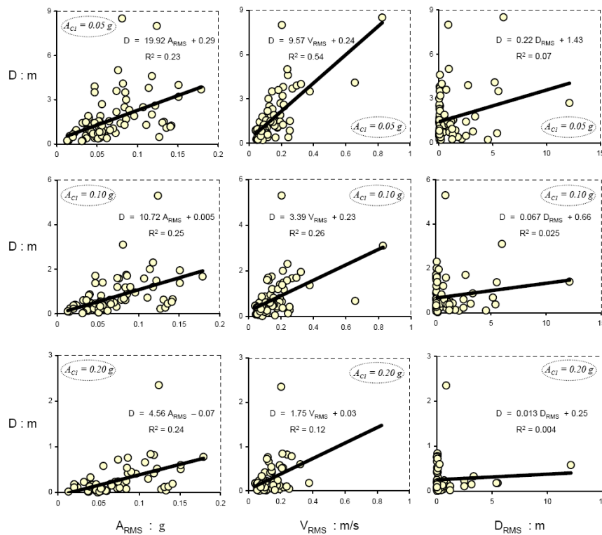
Figure 6. Slippage, D , in connection with the Root Mean Square values: (a) RMS acceleration—in the first column from the left, (b) RMS velocity—in the second column, and (c) RMS displacement—in the last column to the left
