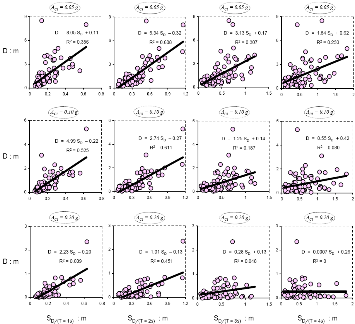
Figure 8. Correlation of slippage, D , with its corresponding spectral displacement at four different periods, T : for period of 1, 2, 3, and 4 seconds
