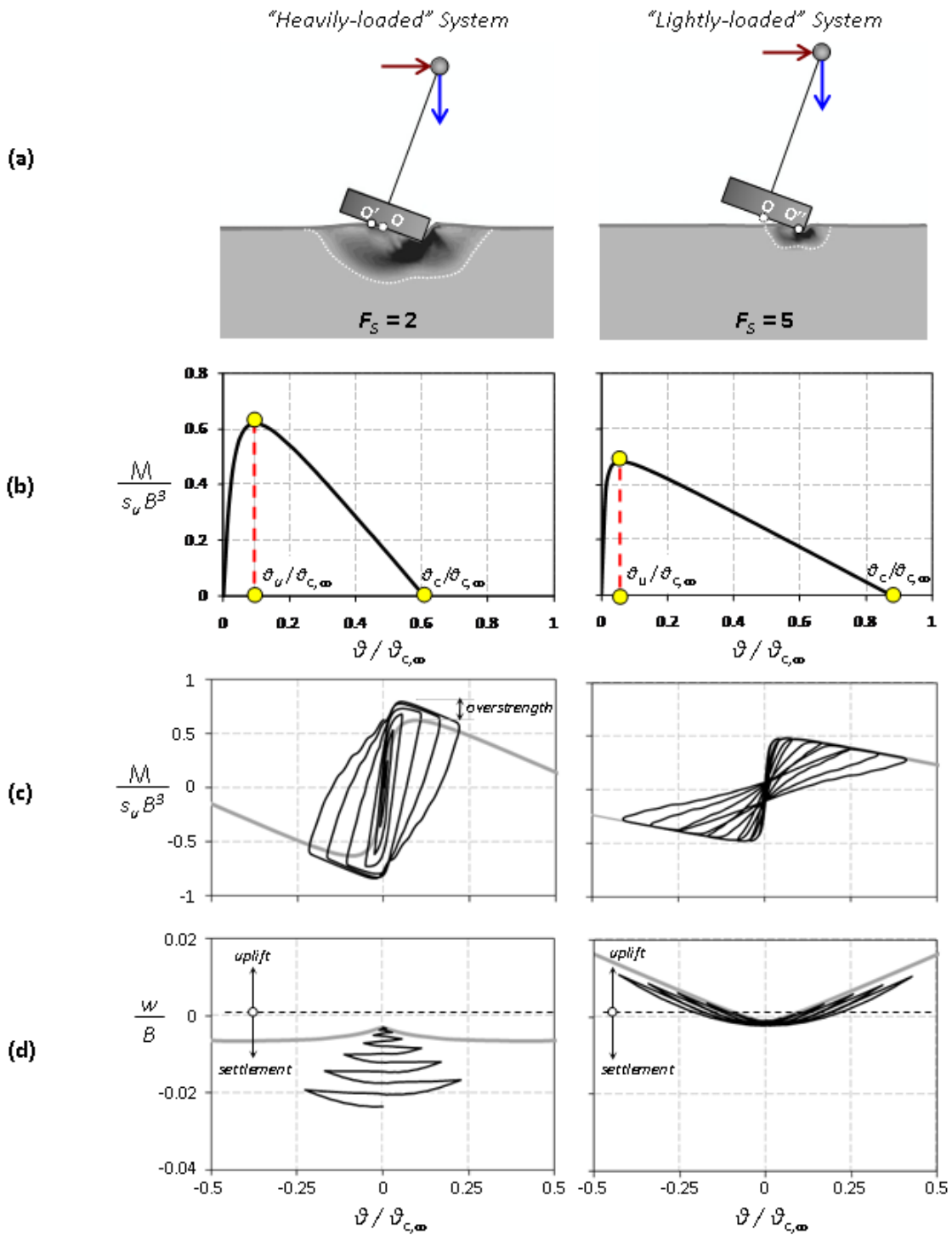
Figure 4. Comparison of two slender systems (differing only in F_S ) subjected to monotonic and cyclic loading: (a) deformed mesh with plastic strain contours at ultimate state; (b) dimensionless monotonic moment-rotation response; (c) cyclic moment-rotation response; and (d) cyclic settlement-rotation response (the grey line corresponds to the monotonic backbone curves).
