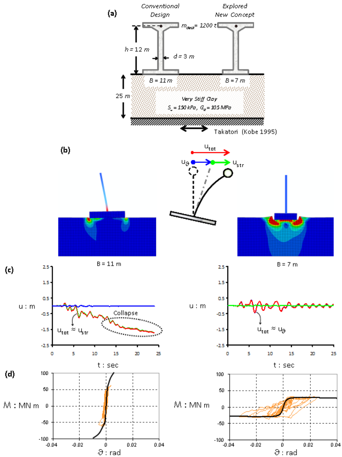
Figure 5. (a) Two bridge piers on two alternative foundations subjected to a large intensity shaking, exceeding the design limits; (b) deformed mesh with superimposed plastic strain, showing the location of “plastic hinging” at ultimate state; (c) time histories of deck drift; (d) overturning moment–rotation ( M – \theta ) response of the two foundations.
