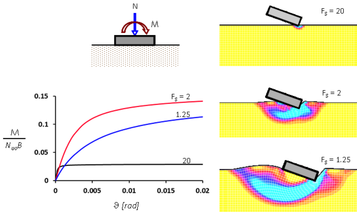
Figure 2. Typical moment–rotation relations of three foundations and corresponding snapshots of their ultimate response with the contours of plastic deformation. The only difference between foundations : their static factor of safety.
