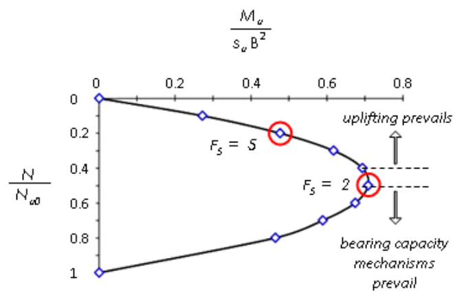
Figure 3. Dimensionless N_u - M_u failure envelope for strip foundation
